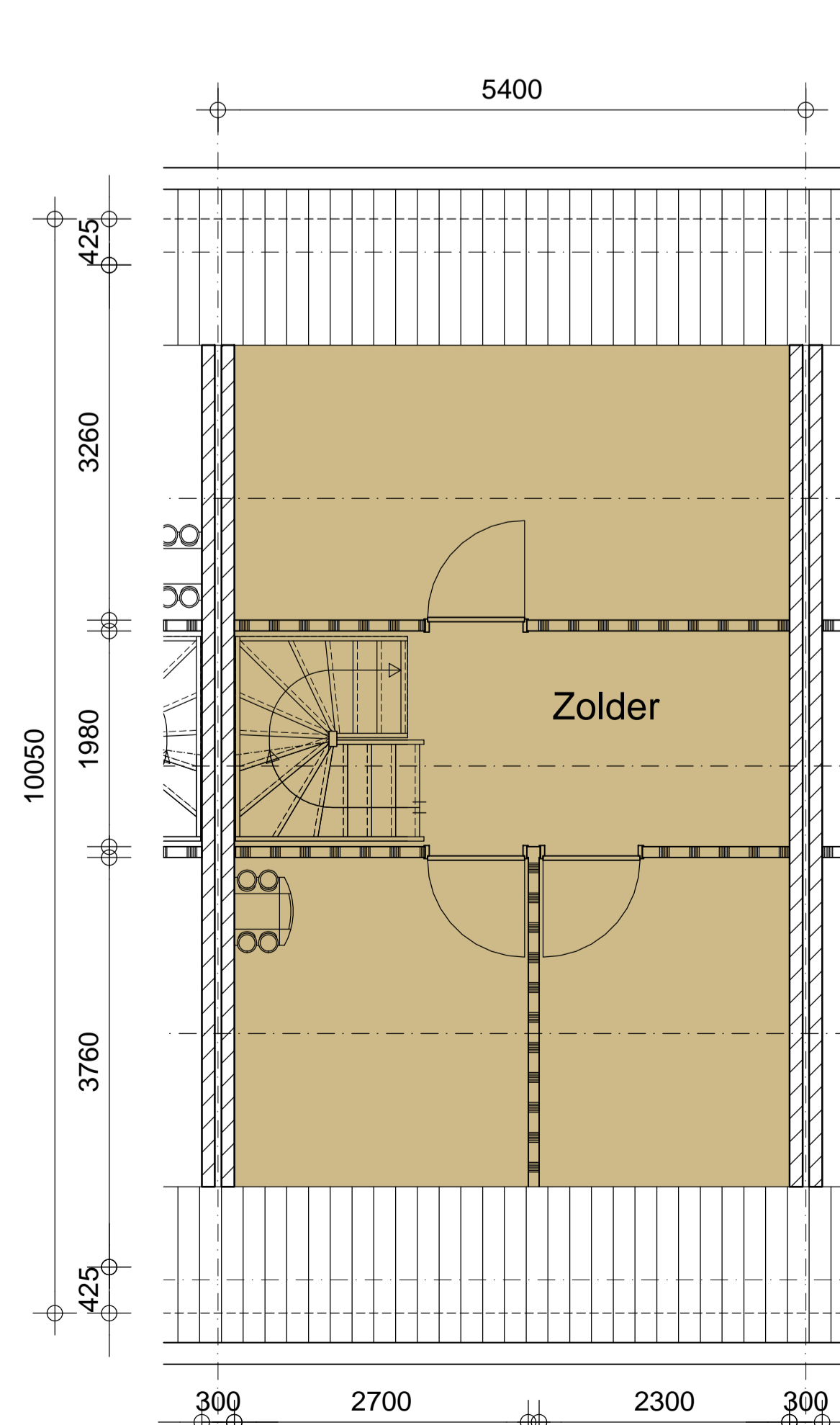
Zolder
